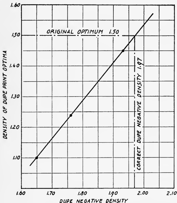
FIG. 10. Curve of print optima vs. dupe negative density. All negatives printed from a dupe positive density of 2.05.
